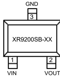
SOT23-3(B-Type)
